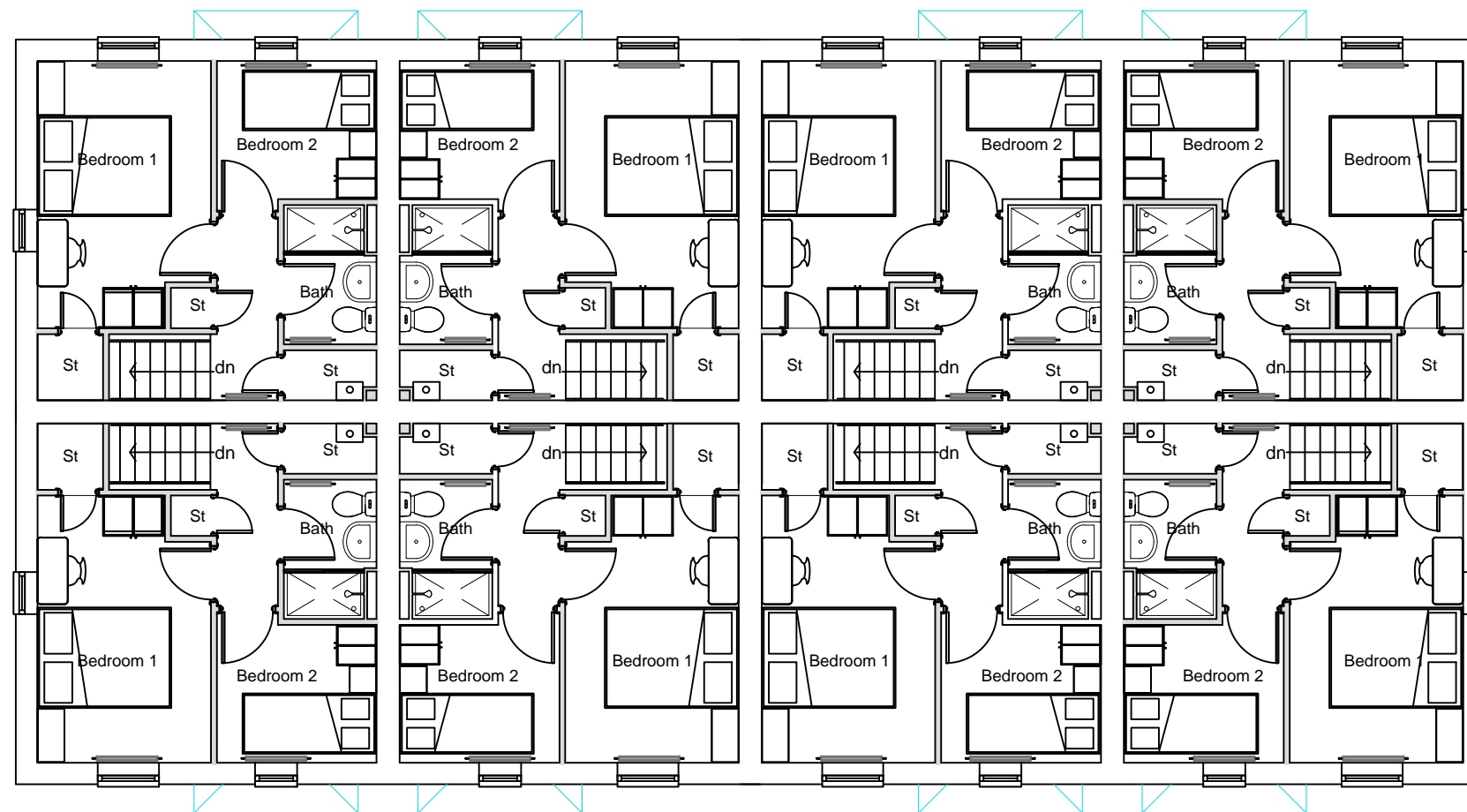
FIRST FLOOR PLAN Type Acomb (end/mid)
